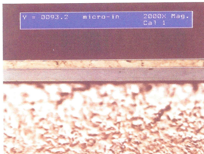
Figure 1-Very thick Au deposit which will undoubtedly result in poor solder connection.
